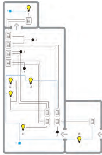
Traditional installation with hard-wired and static spots
